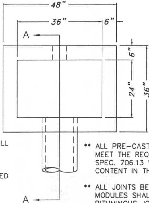
TOP VIEW (CASTING REMOVED)
